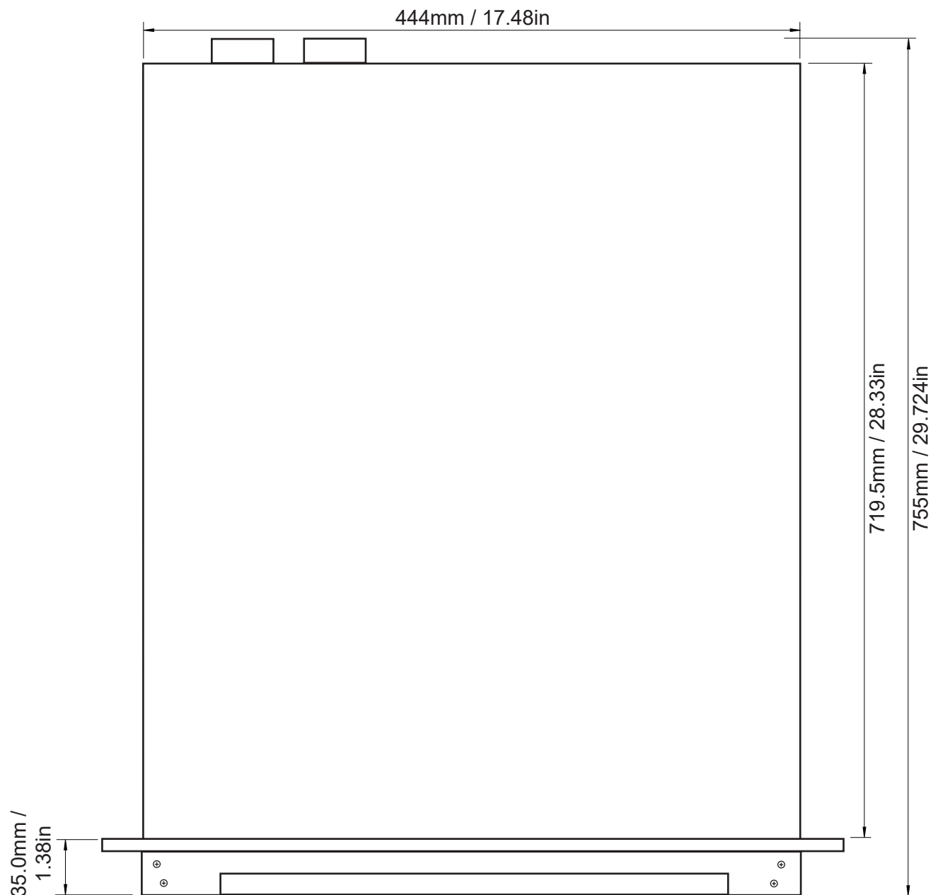
View on Top Face 483mm / 19.02in
