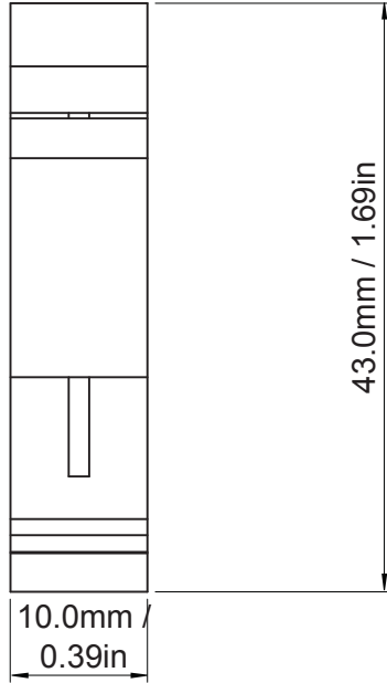
View on Front Face
